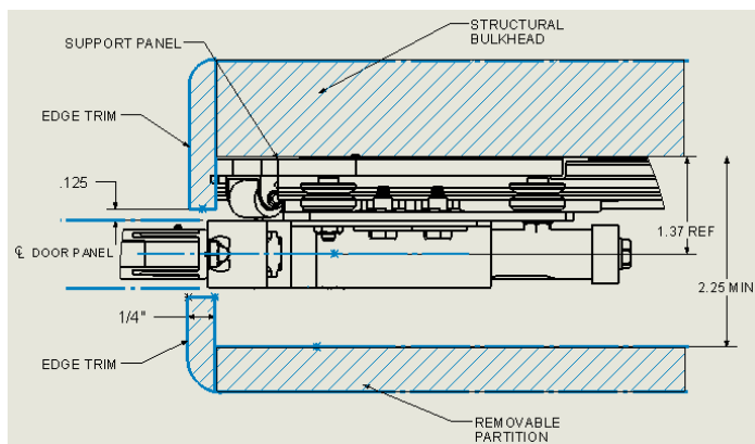
3519-153-1 MECHANICAL DOOR PLAN VIEW
